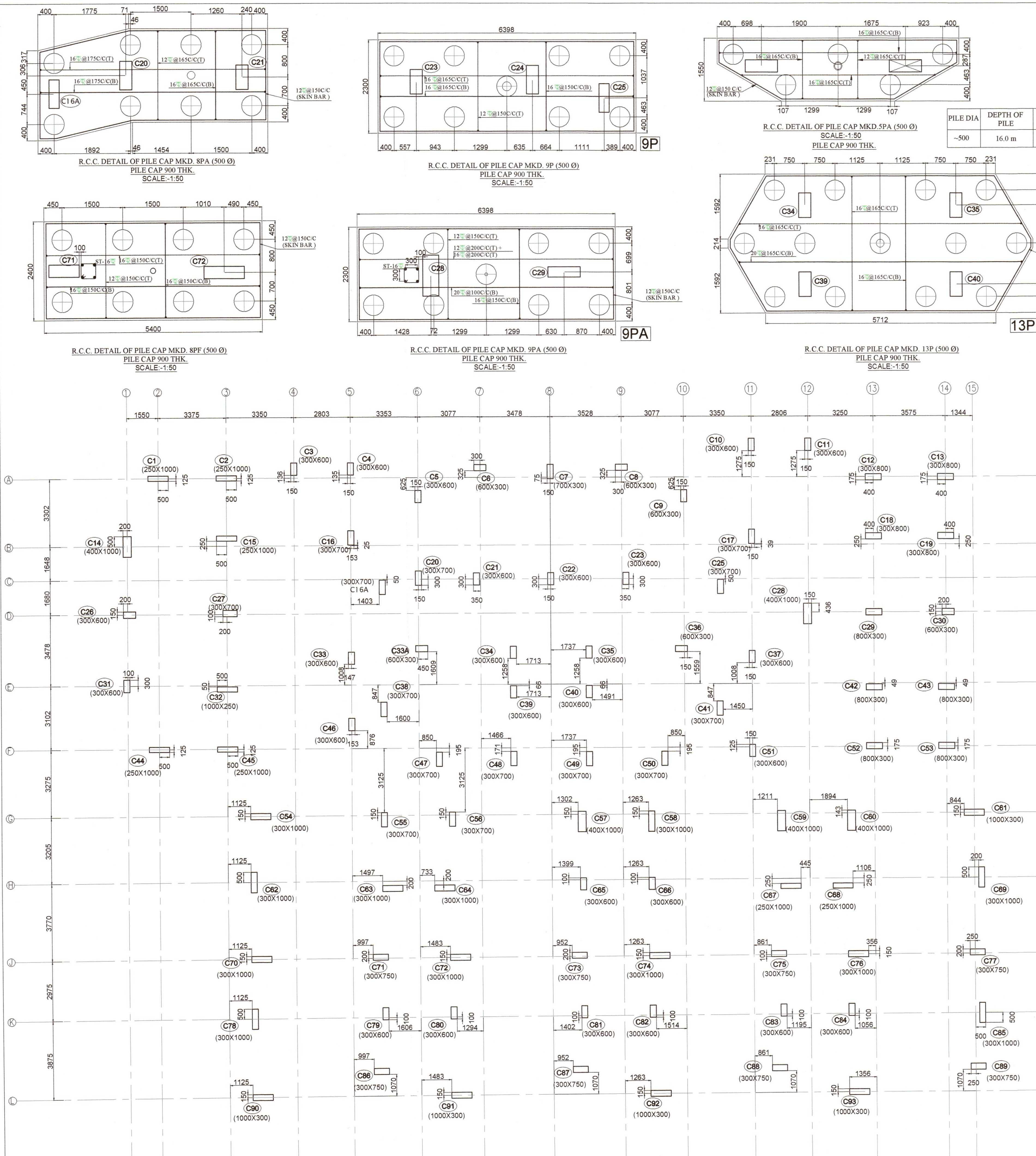
COLUMN LAYOUT PLAN (GROUND FLOOR) SCALE:-1:100
